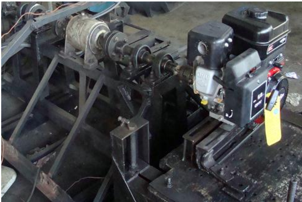
Figure 2. Test set-up of the BRIGGS & STRATTON 122362 Gasoline Engine w/ Gear Reduction.
