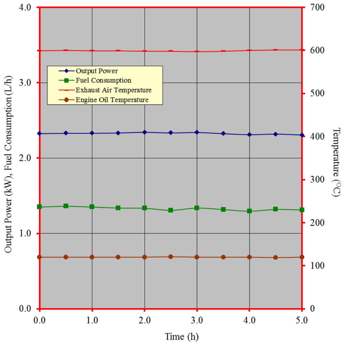
Figure 4. Performance characteristic curves during the continuous running test of the BRIGGS & STRATTON 122362 gasoline engine w/ Gear Reduction
