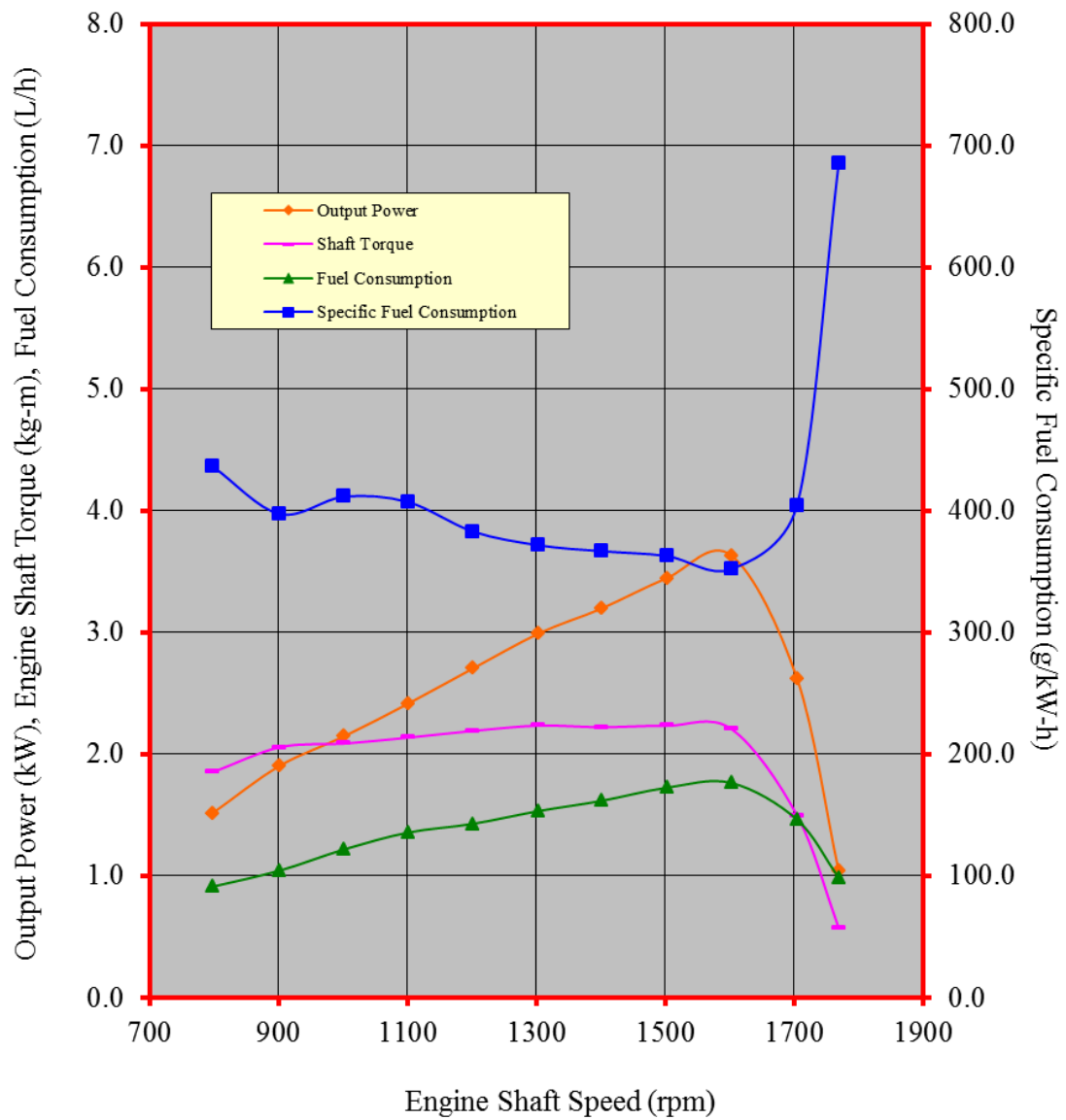
Figure 3. Performance characteristic curves of the BRIGGS & STRATTON 122362 gasoline engine w/ Gear Reduction
